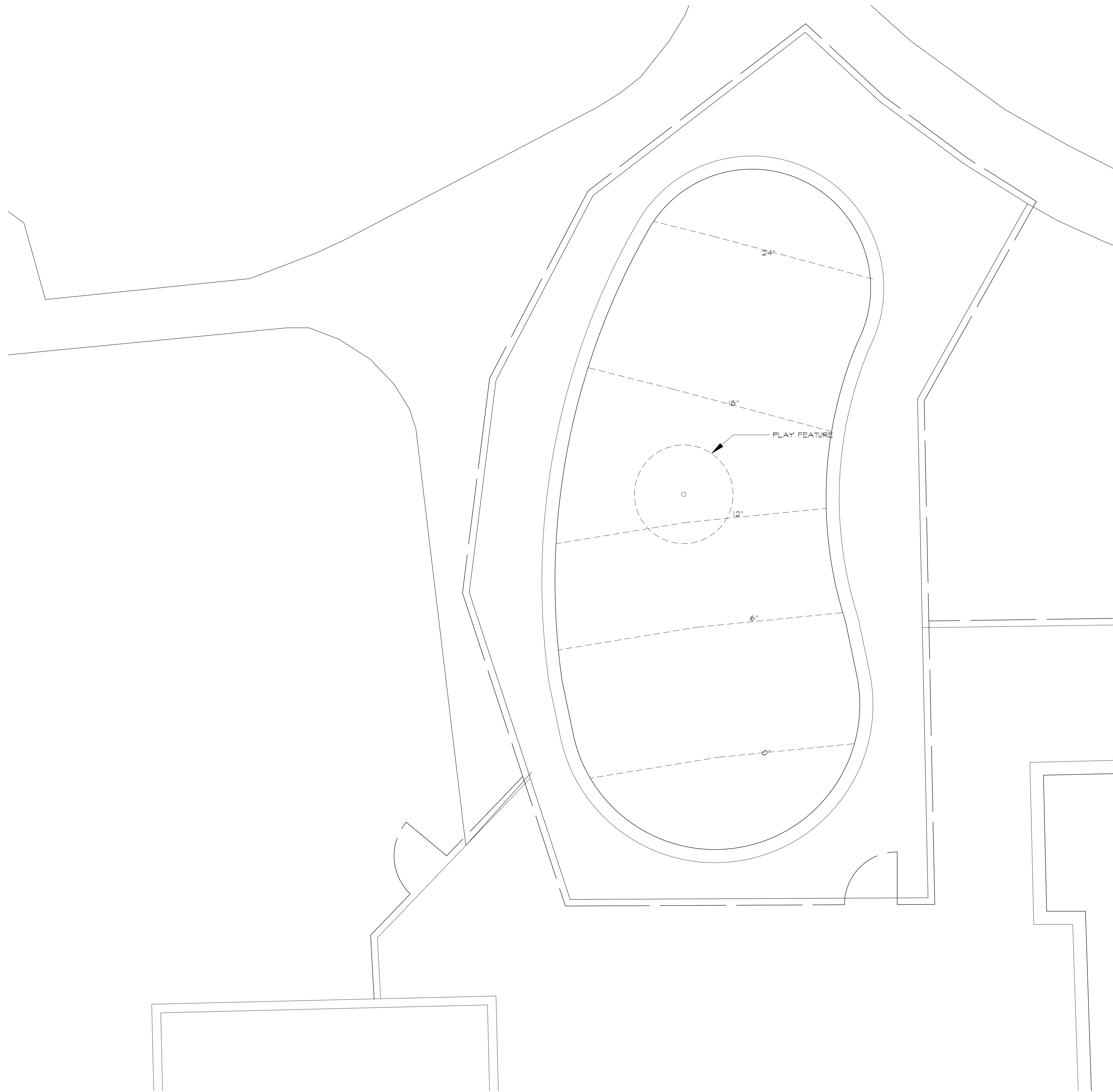
1 POOL PLAN SP-1 1/4" = 1'-0"
